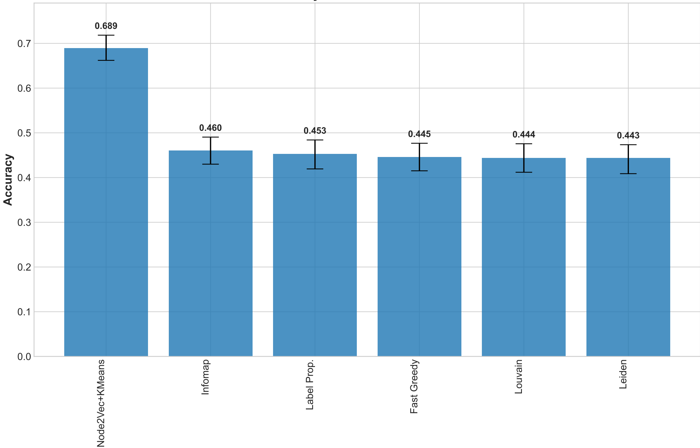
Model Accuracy with 95% Confidence Intervals
